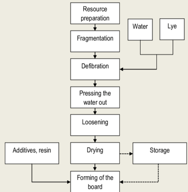
Fig 2: Flowchart illustrating the production process of straw panel
